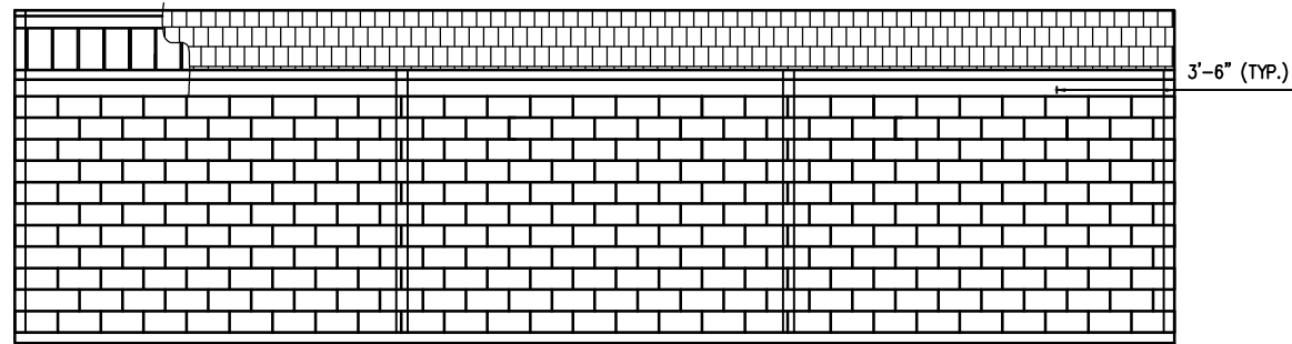
DUGOUT REAR ELEVATION
