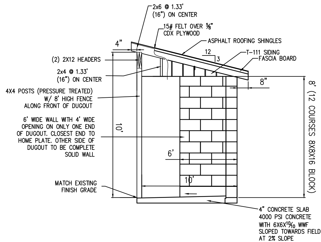
DUGOUT SIDE VIEW
