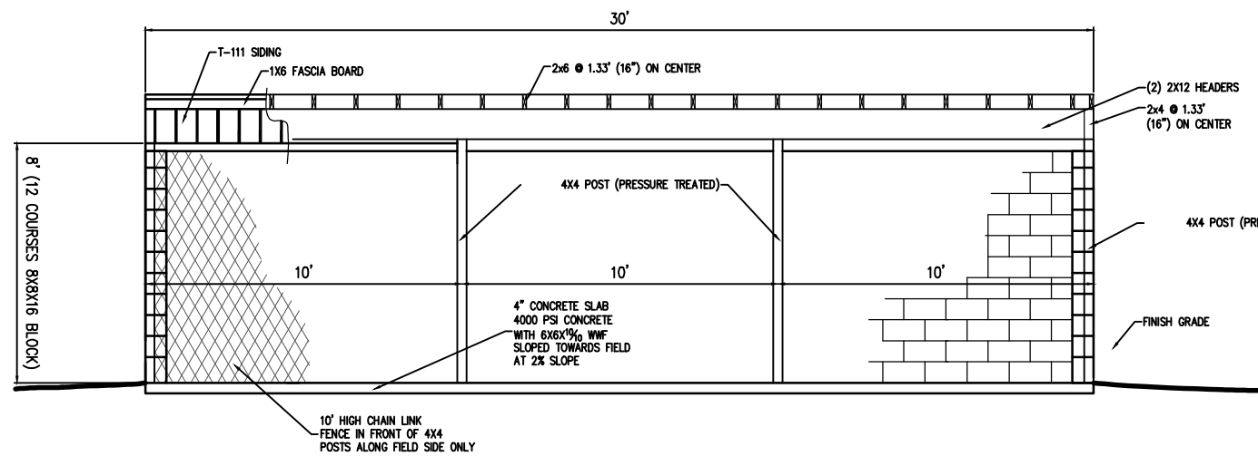
DUGOUT FRONT ELEVATION
