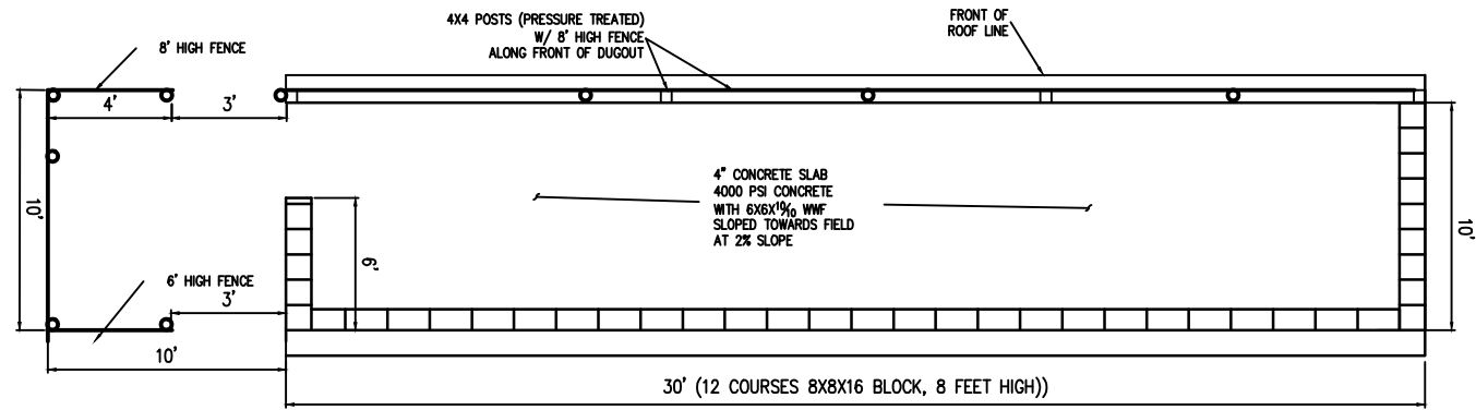
DUGOUT PLAN ELEVATION
